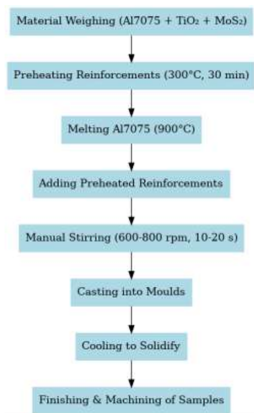
Fig. 1 Fabrication process flow diagram
